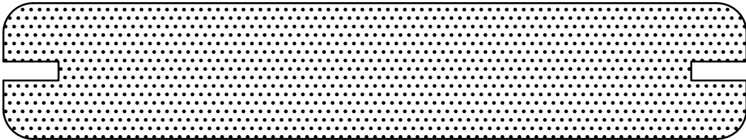
5/4x6 RADIUS EDGE DECKING - GROOVED 1"x5-1/2" PVC
