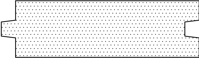
1x4 FLOORING PVC 3-1/4" FACE 3-1/2" OVERALL
